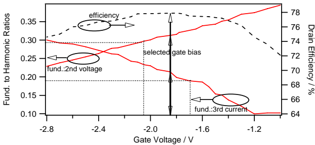
Fig. 1. Gate sweep at 28V drain voltage bias condition at 0.9GHz.
