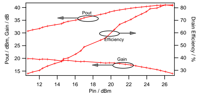
Fig. 5. Power sweep at 28V drain voltage bias condition at 2.1GHz
